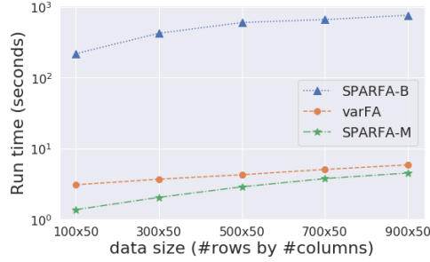
Figure 3.2. Training run time comparing VarFA, SPARFA-M, and SPARFA-B on synthetic data sets of varying sizes. VarFA performs approximate Bayesian inference almost 100x faster than SPARFA-B and is close to the run time of SPARFA-M. Thus, VarFA enables practical and scalable Bayesian inference for very large data sets.
